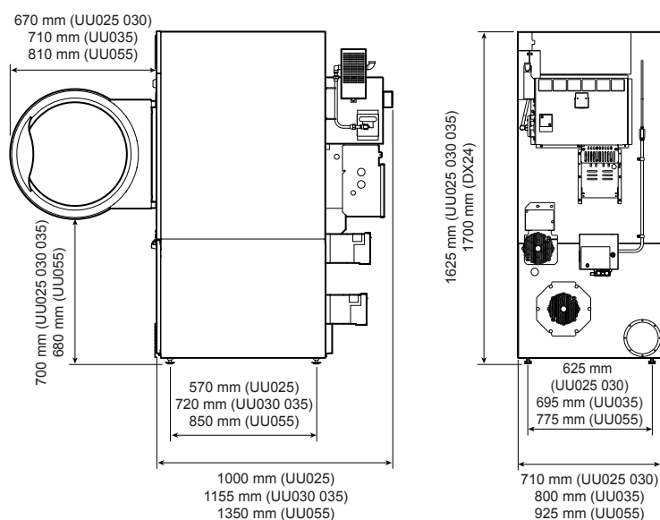
LATERAL UU025, UU030, UU035, UU055
